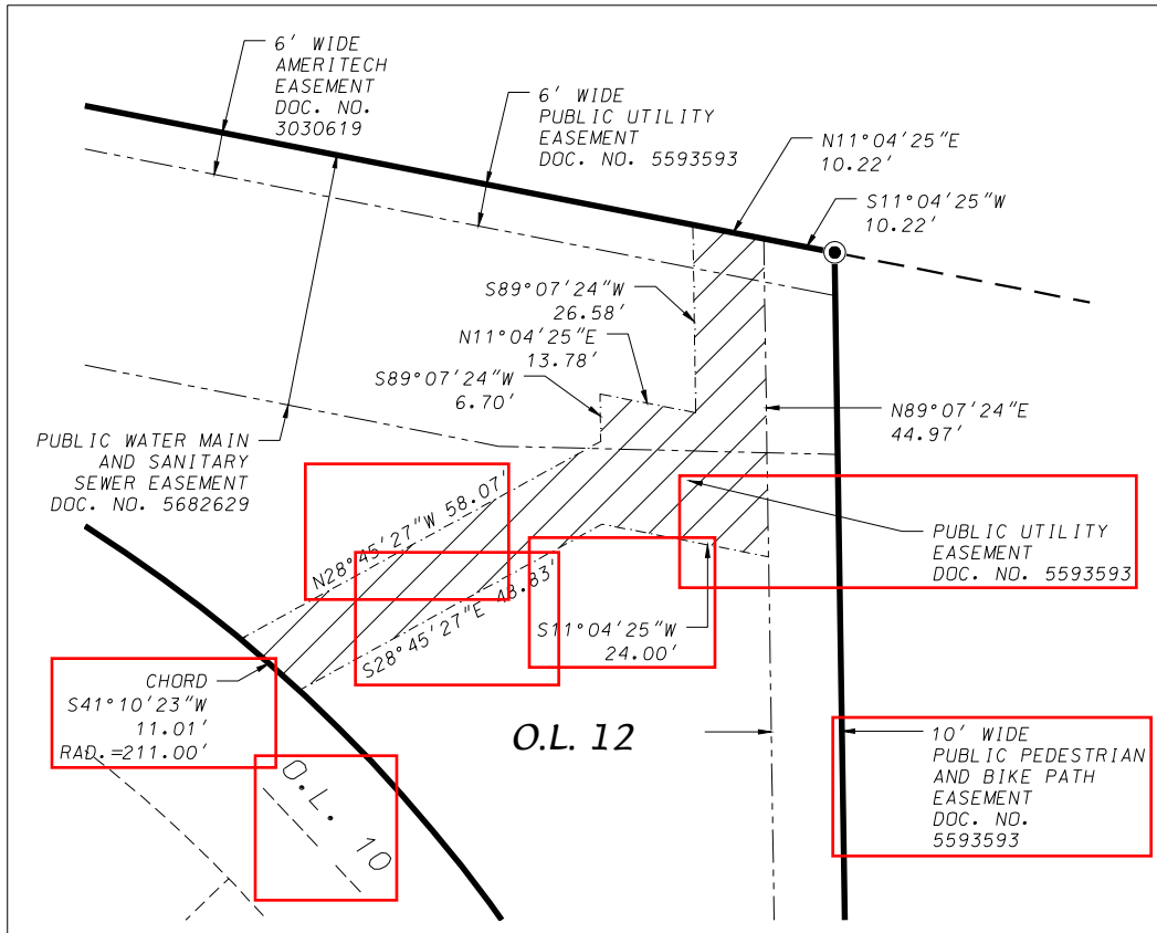
PUBLIC UTILITY EASEMENT DOC. NO. 5593593 - DETAIL
